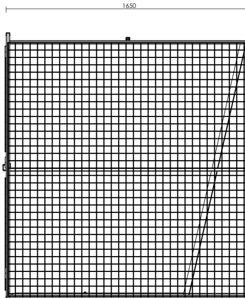
Side View
