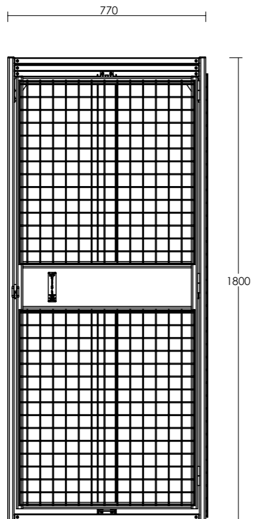
Front View
